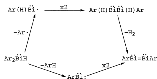
Scheme 1. Two possible mechanisms for the transformation of Ar 2 BiH to ArBi=BiAr (Ar = 2,6-Mes 2 C 6 H 3 ).
